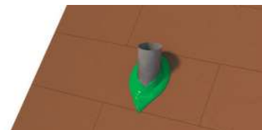
Sealing the pipe in one go (wrap around PAVATAPE FLEX). Don't forget to prime!
